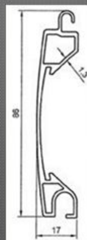
60 mm SLAT: Perforated Pencereleli Z oknom
